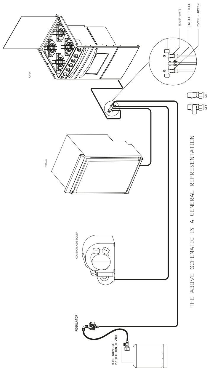
Typical gas schematic drawing with Combi / Alde boiler
